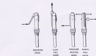
ACTION OF FORCE REQUIRED TO FUNCTION THE SWITCH
