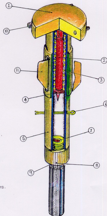
SECTIONED VIEW OF THE SWITCH
