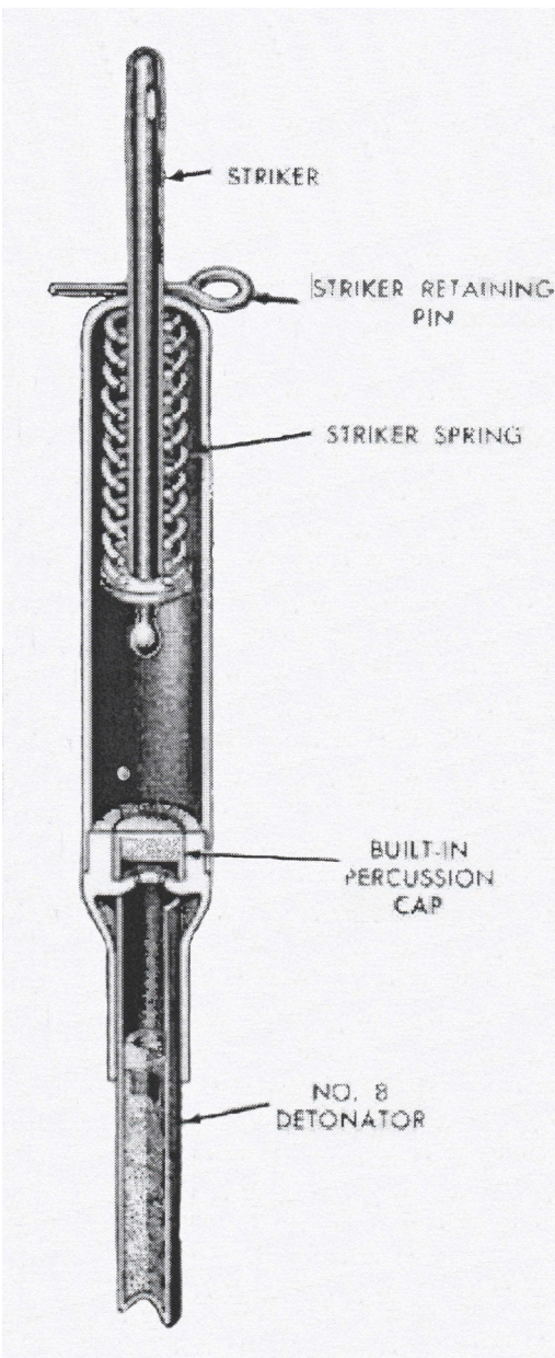
UV Firing Device internal diagram
