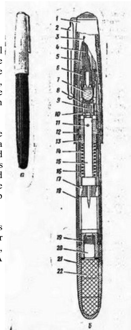
MV-3 Firing Device internal diagram
