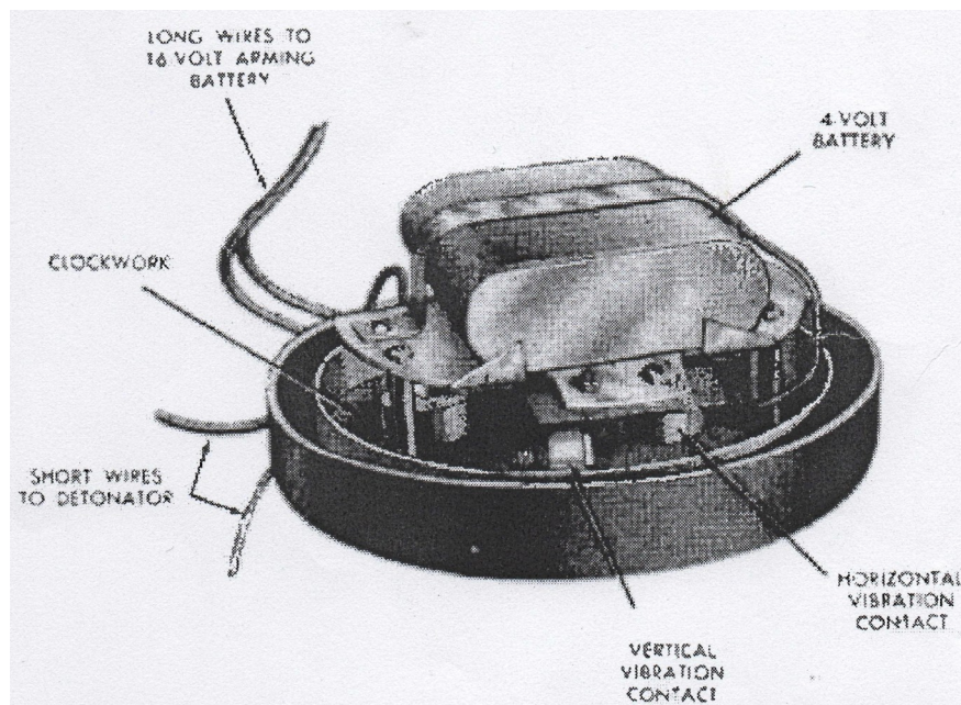
ChVZ showing internal construction
