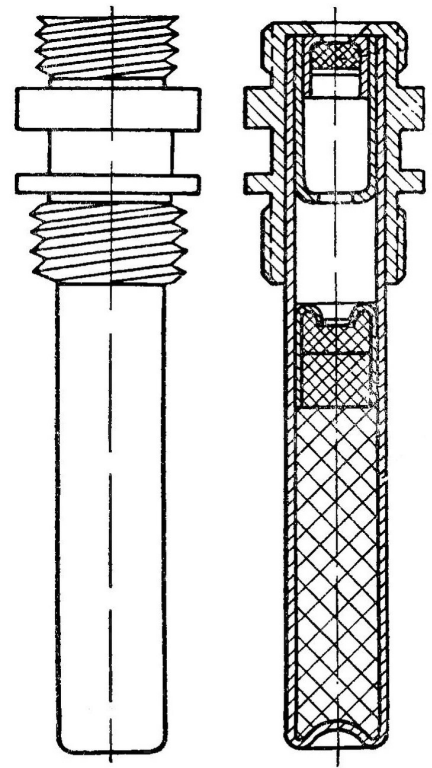
MD-5M Detonator Assembly
