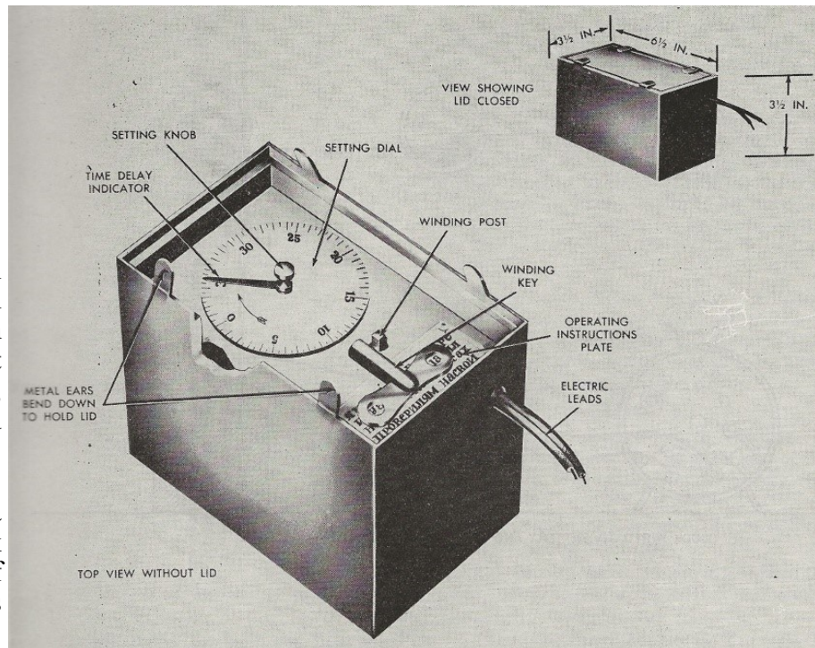
ChZ-35 Rectangular Firing Device
