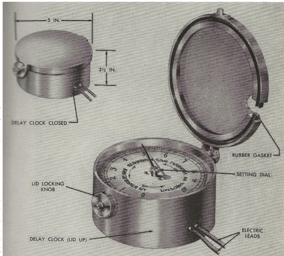
ChZ-10 Firing Device
