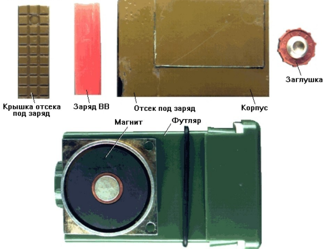
MZD-21 demolition charge components
