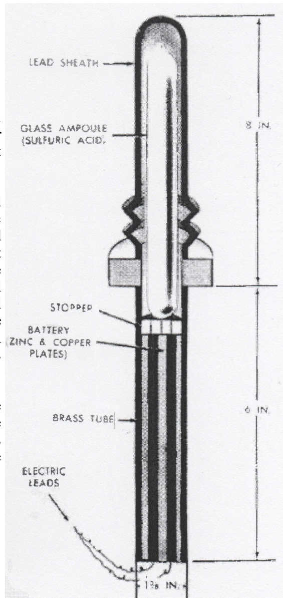
EKhZ Firing Device
