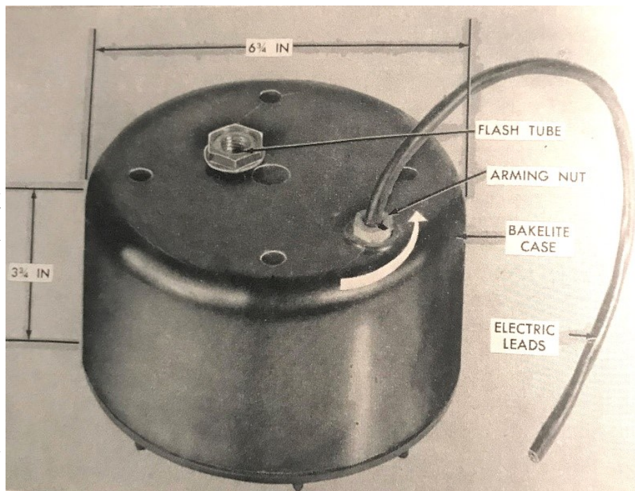
SM-12 Firing Device
