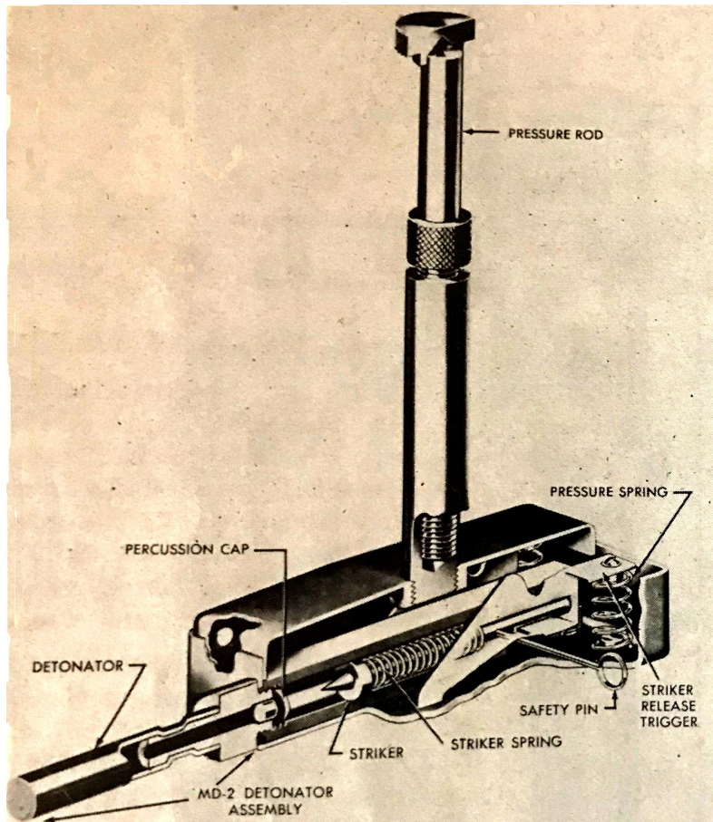
Internal Diagram of the PV-42 Firing Device
