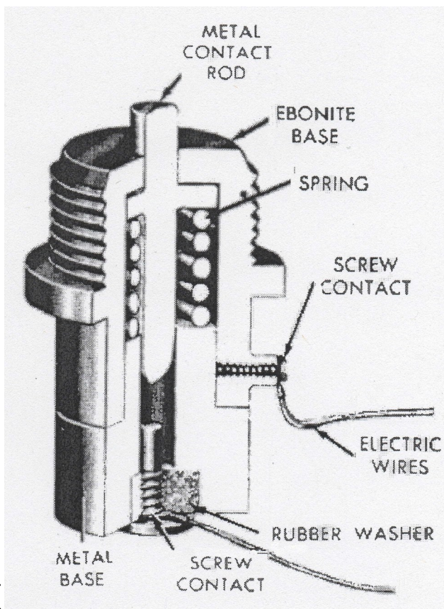
Electrical base for VZDKh
