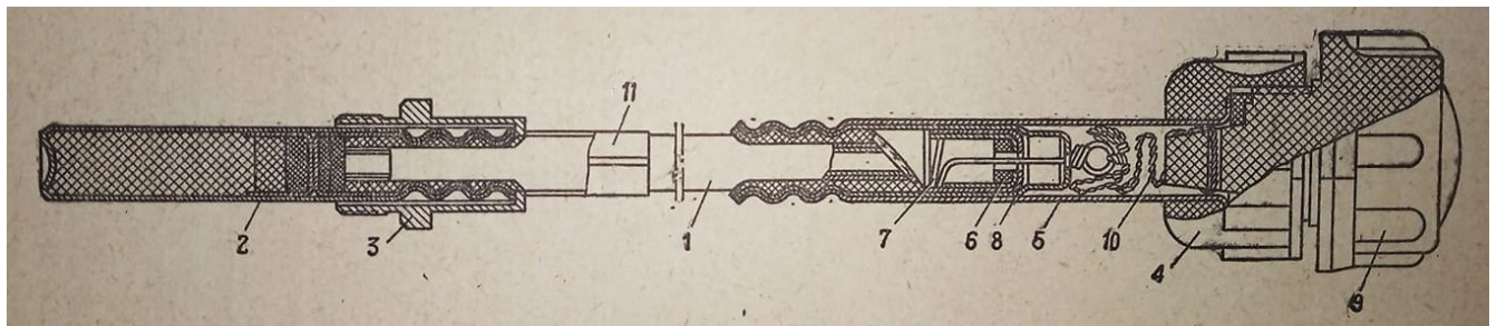
Internal diagram of ZTP-T Friction Lighter on ZTP-50
