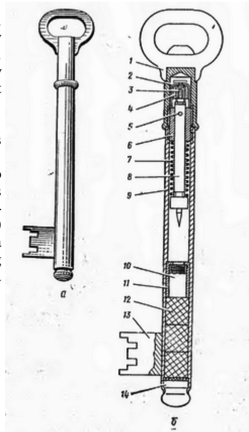
MV-1 internal diagram
