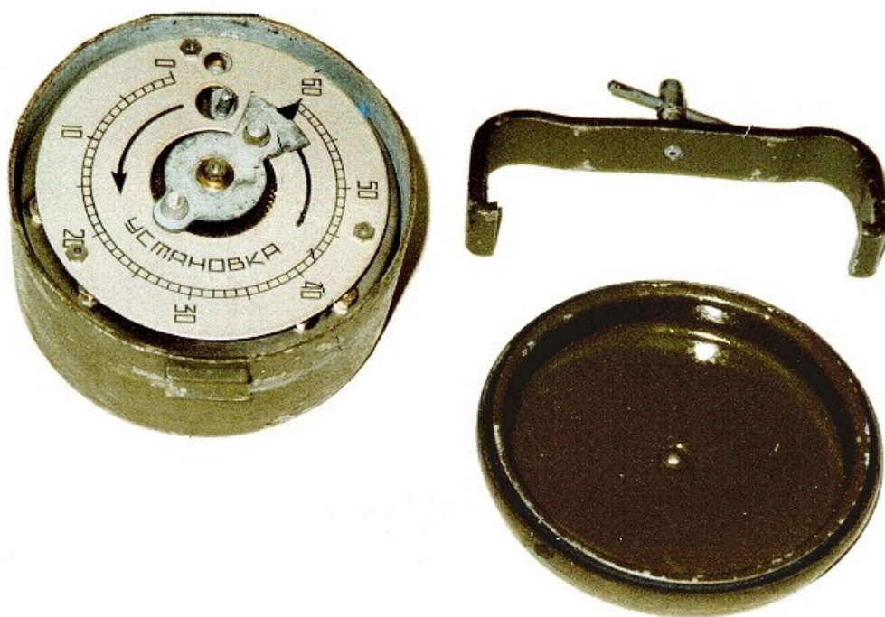
ChMV-60 with cover removed
