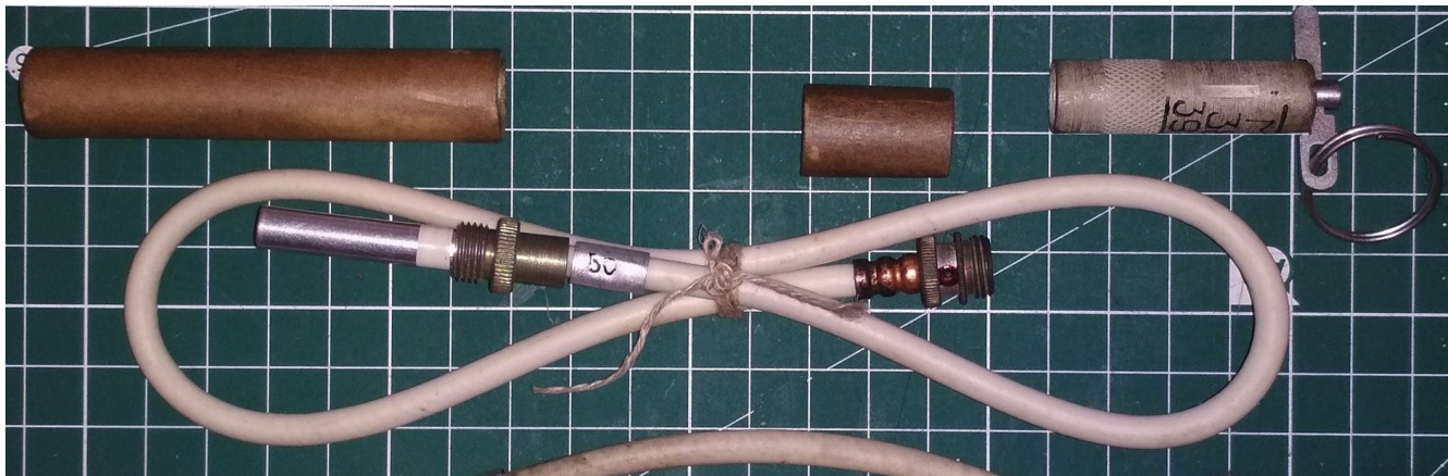
ZTP-M and ZTP-50 Photo- Oleksandr Mariash
