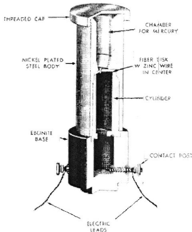
EKhZ Mercury Delay Internal diagram
