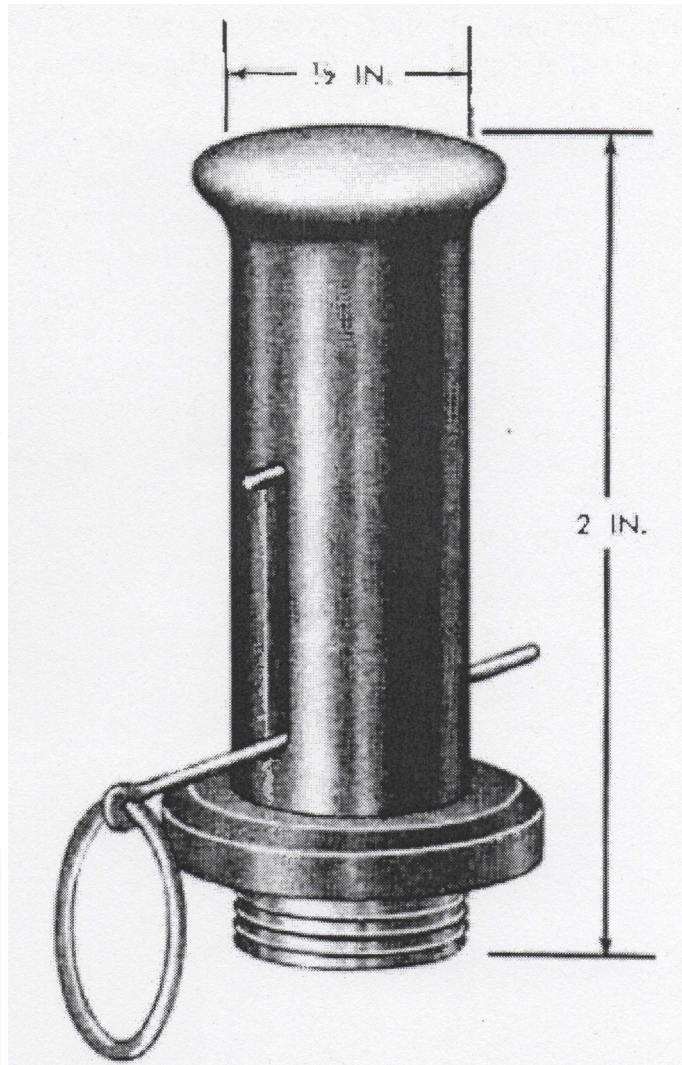
Koveshnikov Firing Device
