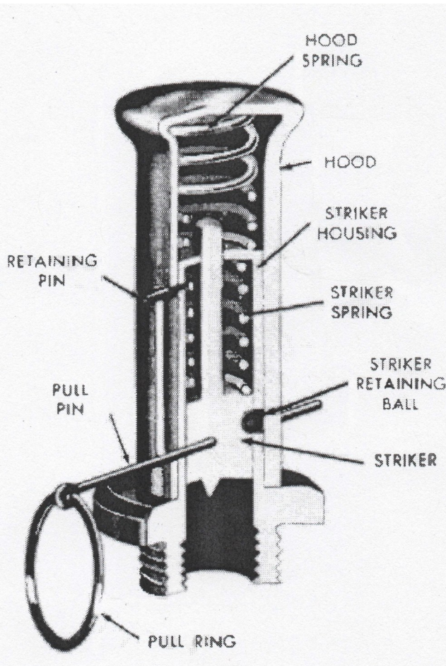
Koveshnikov Firing Device internal diagram
