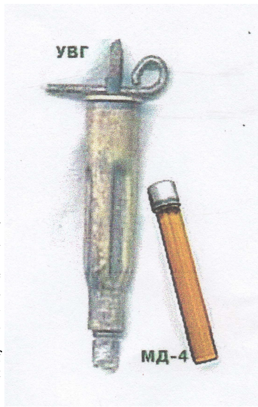
UVG Firing Device
