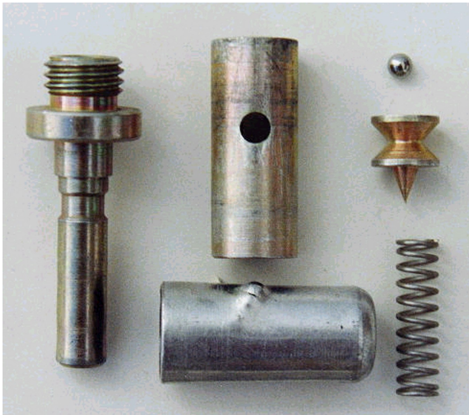
MV-5 Firing device disassembled, note the detonator assembly is a solid training version. Photo- Fenix Insight
