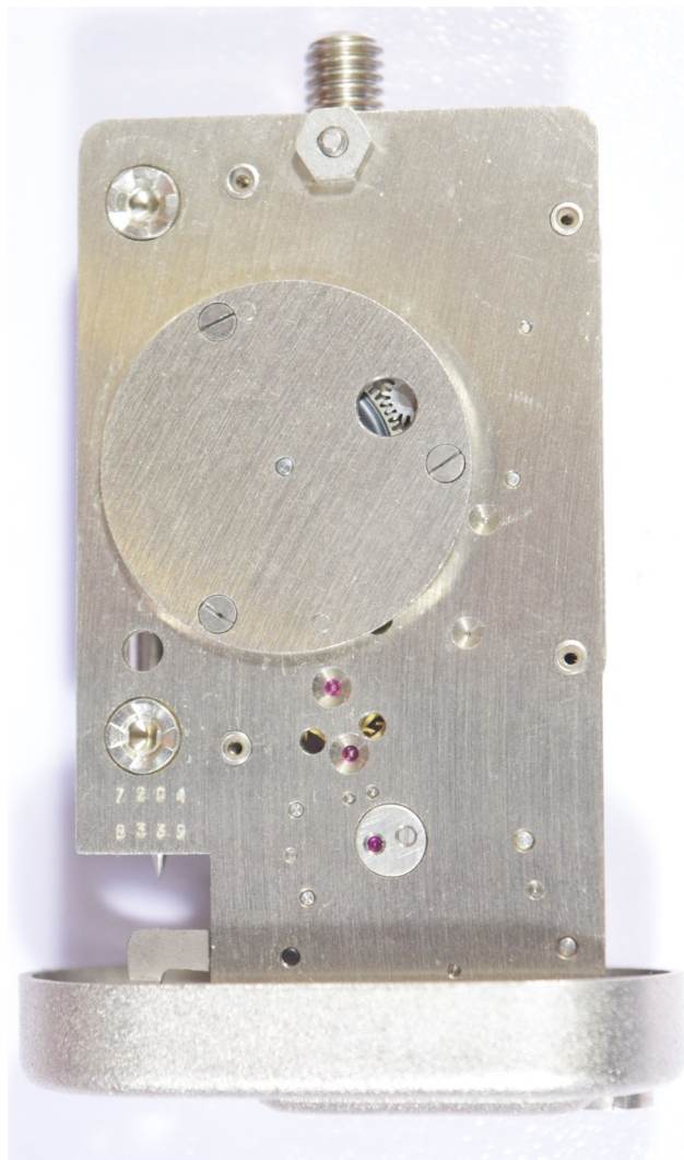
VZD-6Ch Back with casing removed
