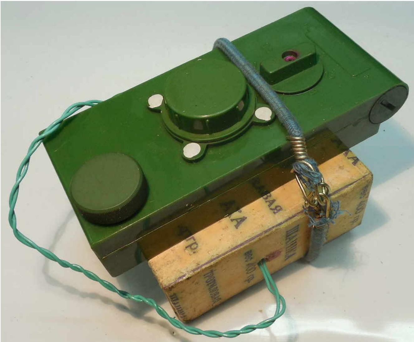
VZDP-16Ch Sensor with attached demolition charge
