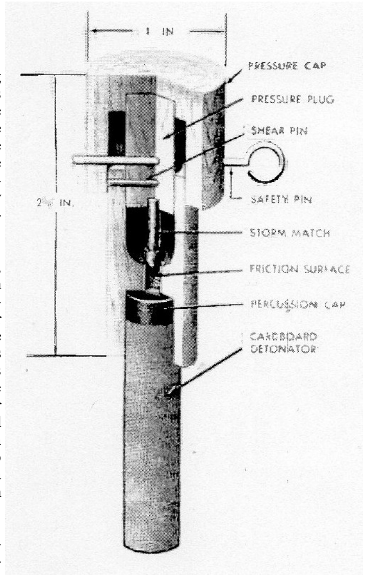
Wooden Pressure Fuze
