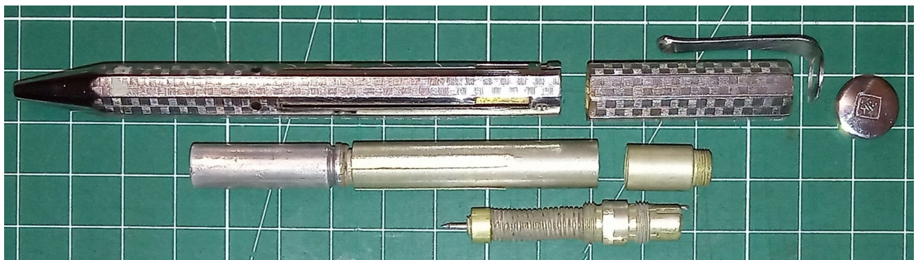
MV-2 Firing device Photo- Oleksandr Mariash
