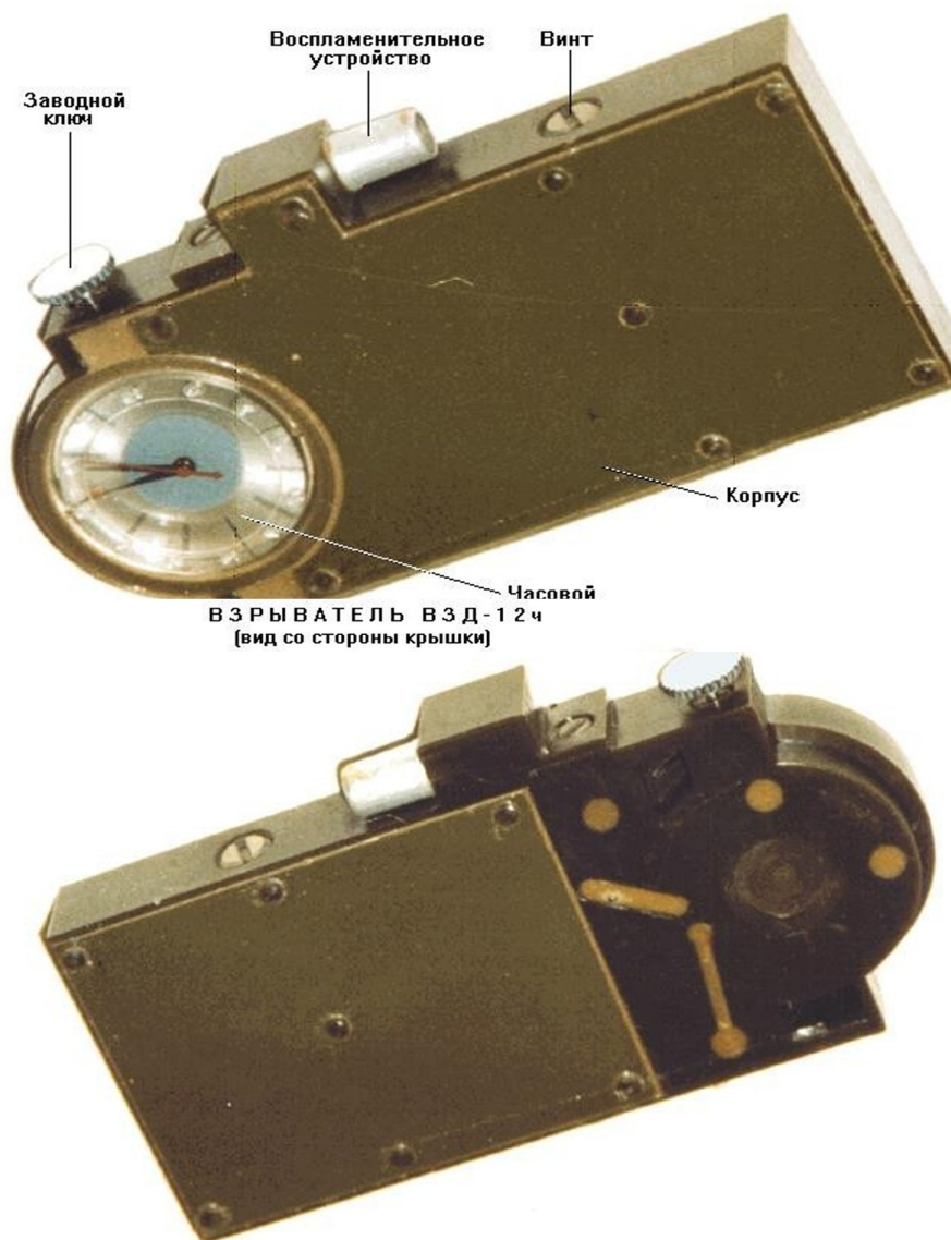
VZD-12Ch Firing Device
