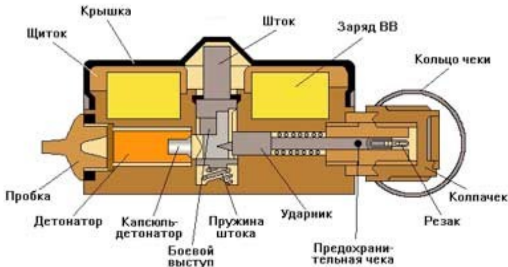
Internal view of the MS-3
