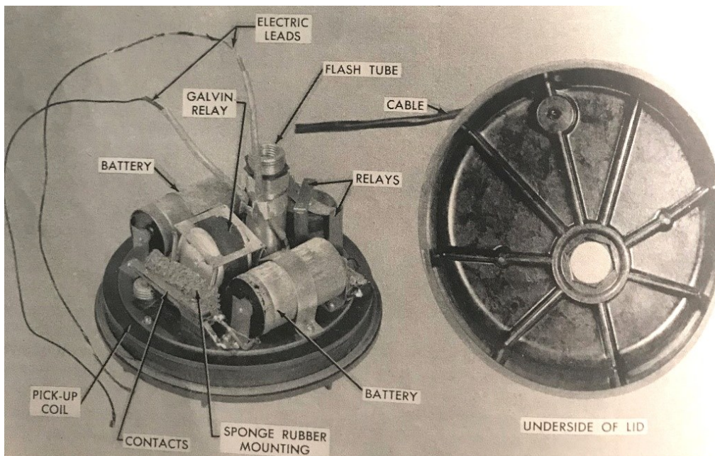
SM-12 with cover removed
