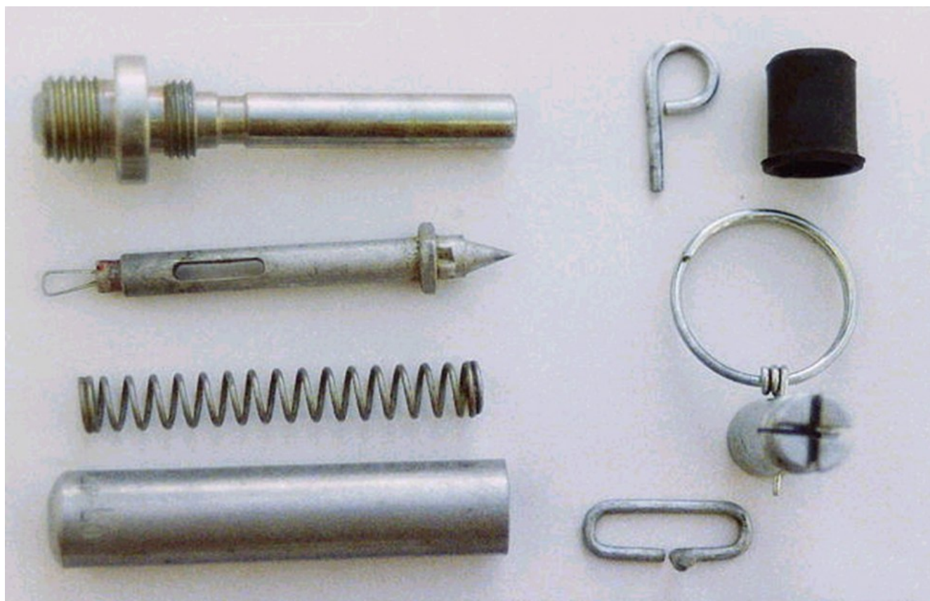
MUV 2 disassembled, note the detonator assembly is an inert training version
