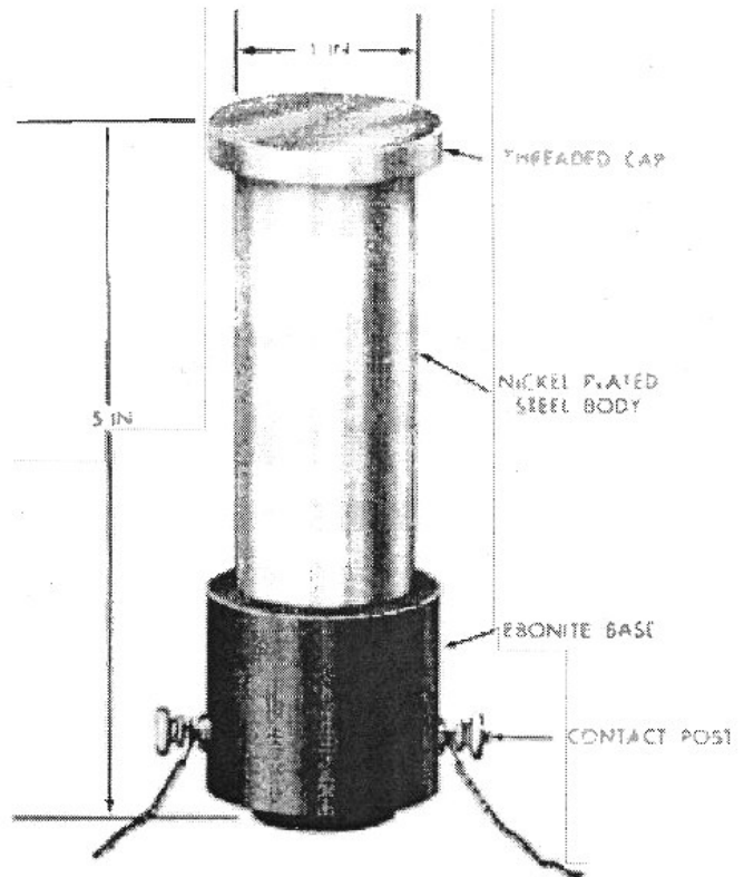
EKhZ Mercury Delay Firing Device
