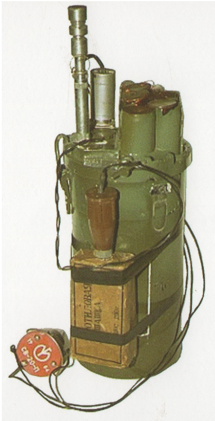
VP13 note the attached demolition charge and MUV-4 firing device.
