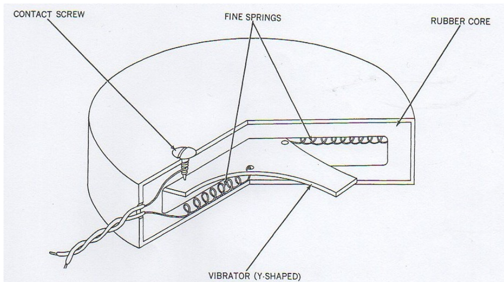
VZ-1 Internal diagram
