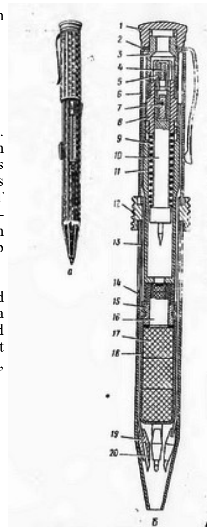
MV-2 Firing Device internal diagram
