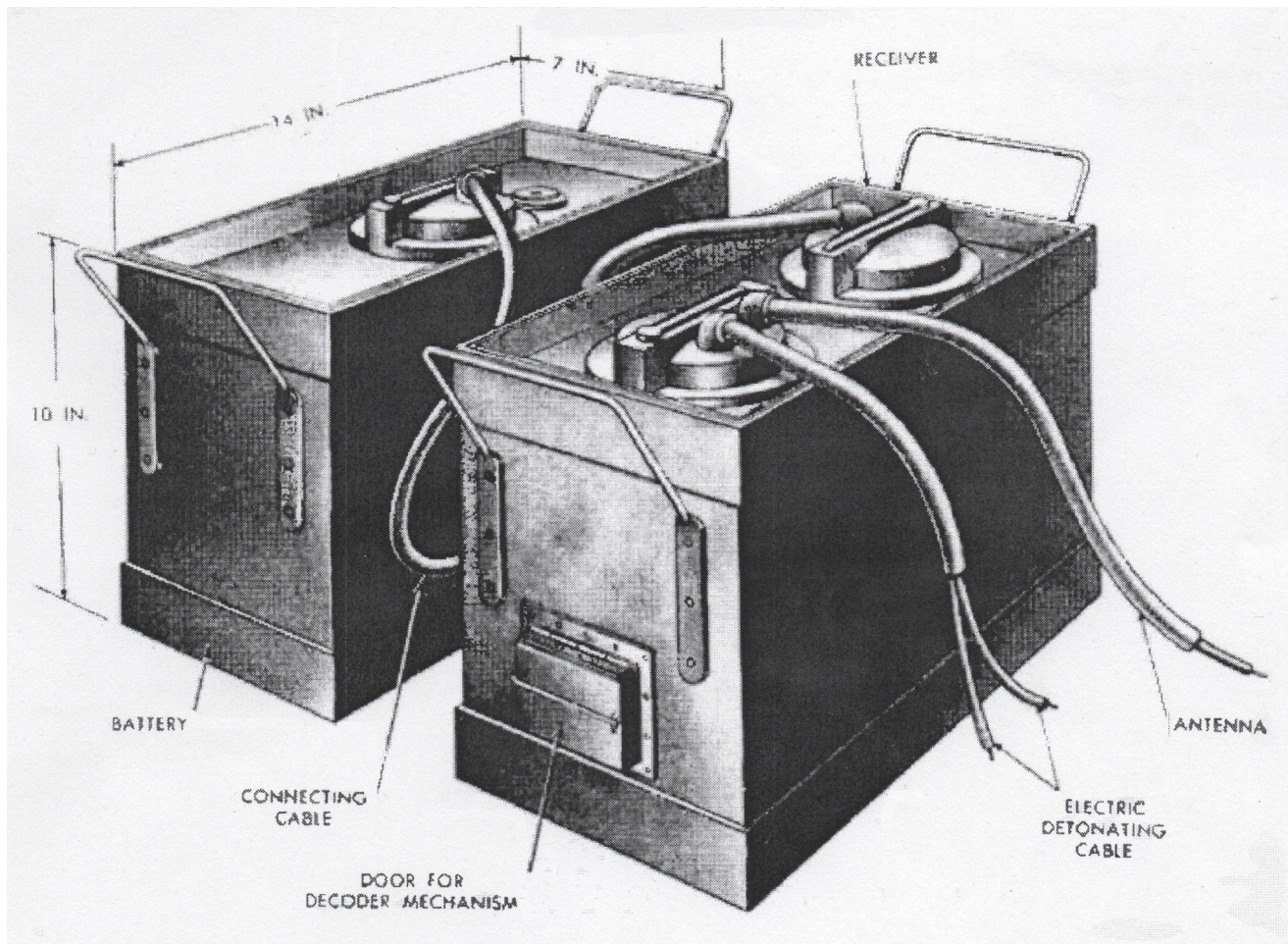
F-10 Firing Device
