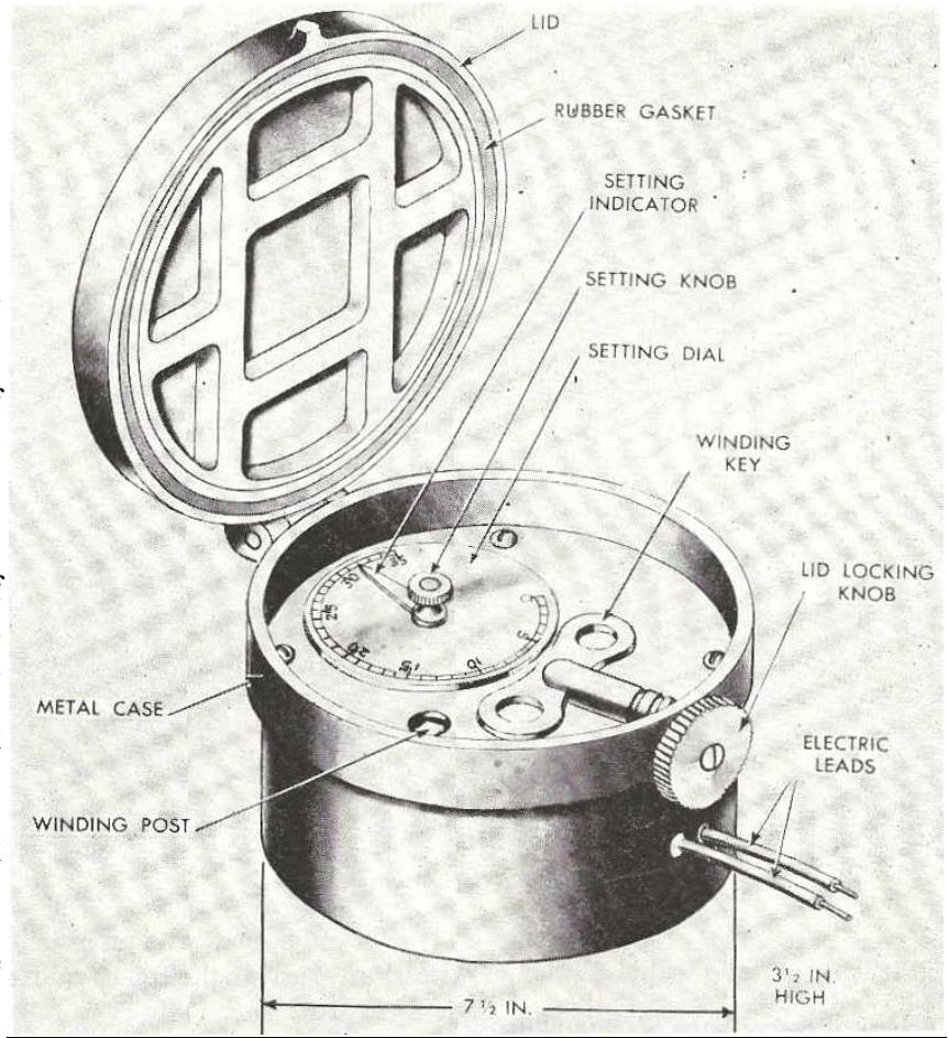
ChZ-35 Cylindrical Firing Device
