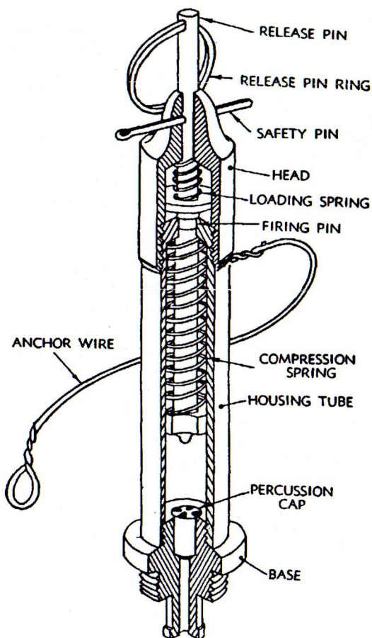
Firing Device, Pull, M1 (Old style) Internal diagram
