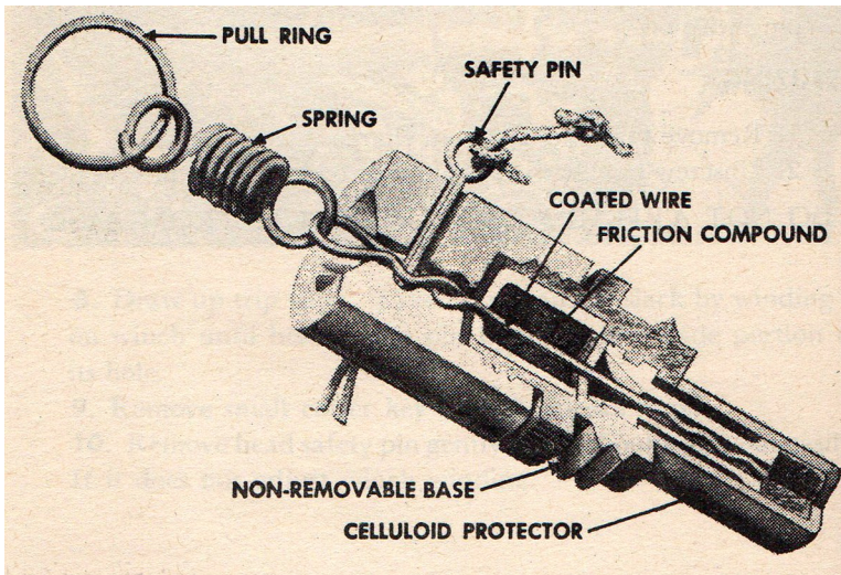
Firing Device, Pull, M2 Internal diagram
