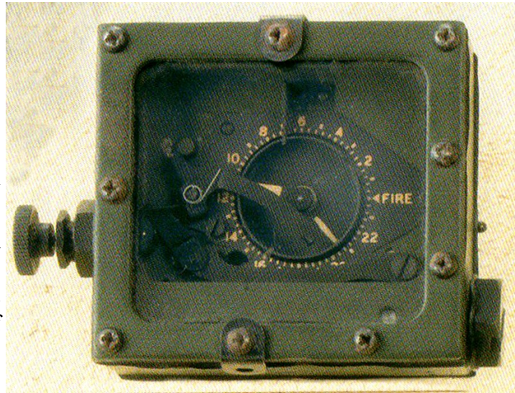
Front of Firing Device, Clockwork, 24 Hour (CIA)
