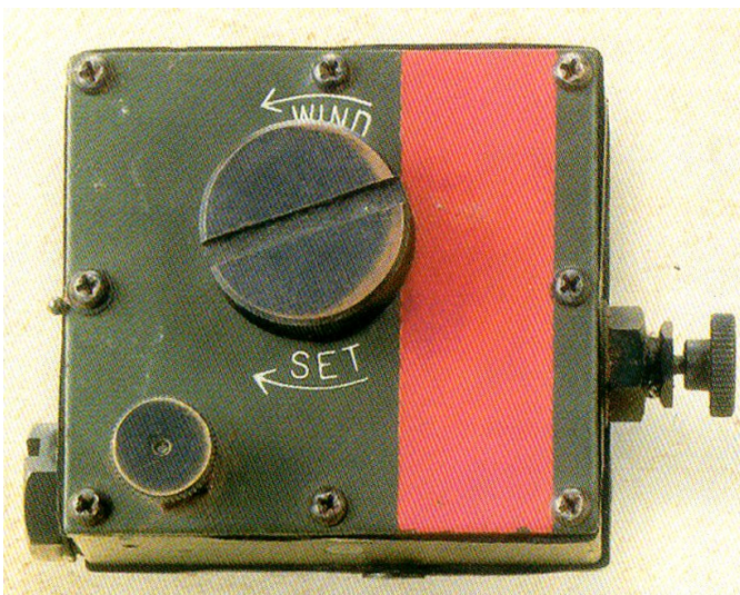
Back of Firing Device, Clockwork, 24 Hour (CIA)
