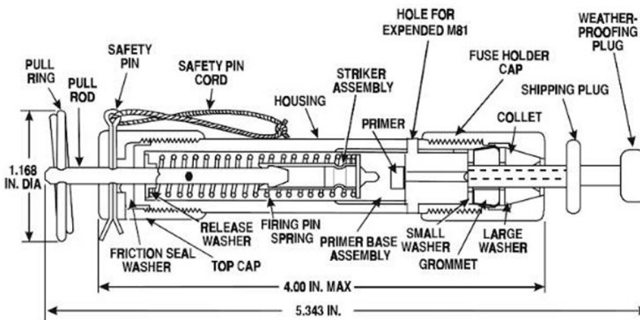
Igniter, Time Blasting Fuse, M81 internal diagram
