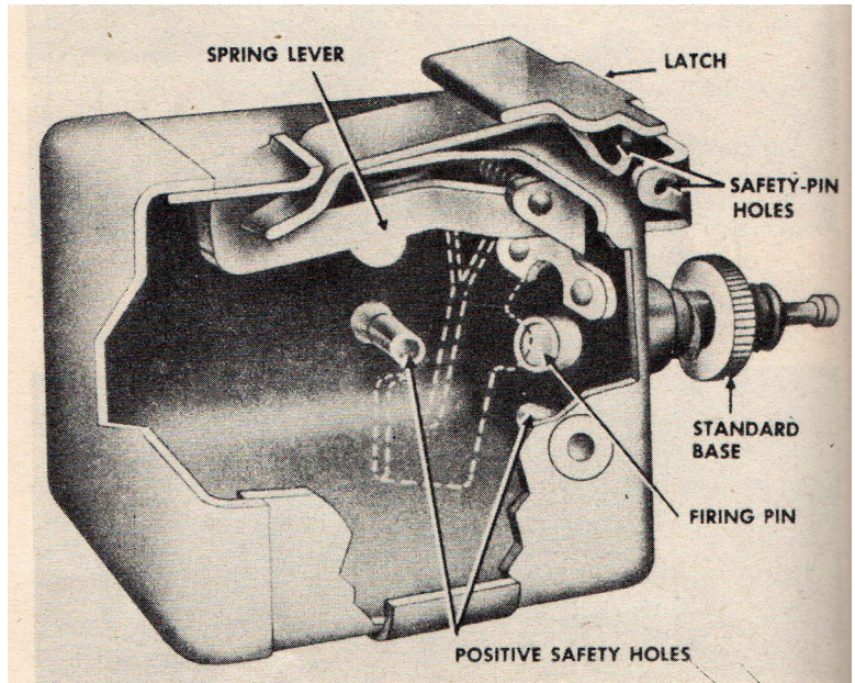
Firing Device, Release, M1 (old style) internal diagram
