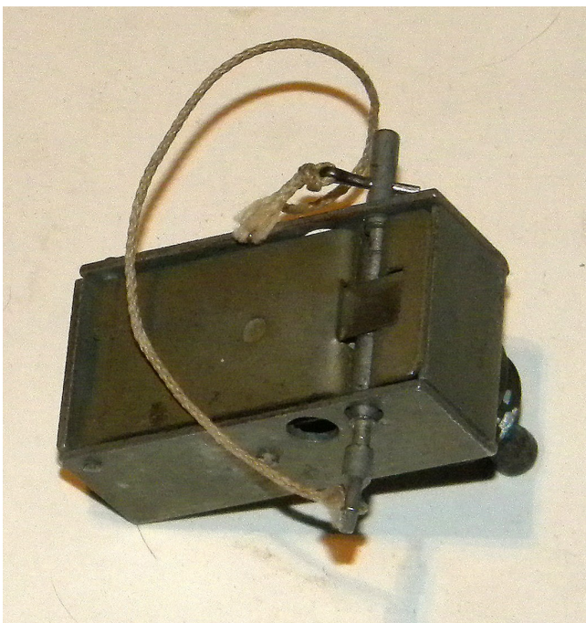
Firing Device, Release, M5
