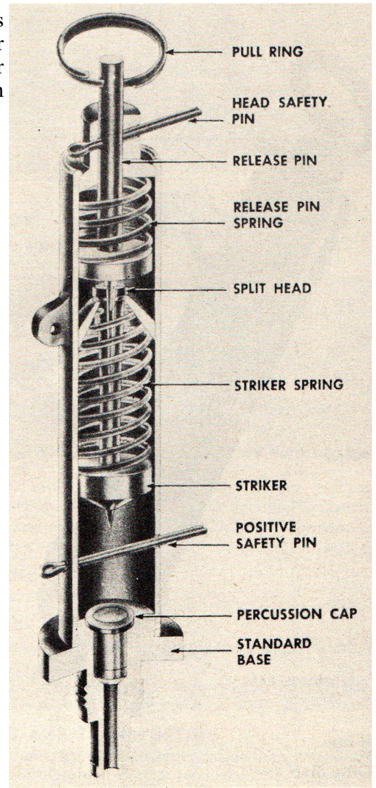
Firing Device, Pull, M1 internal diagram
