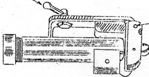
Fig.3. - Pull position.
