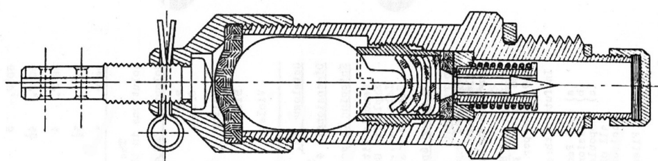
AC Delay, Mk. 1 internal diagram
