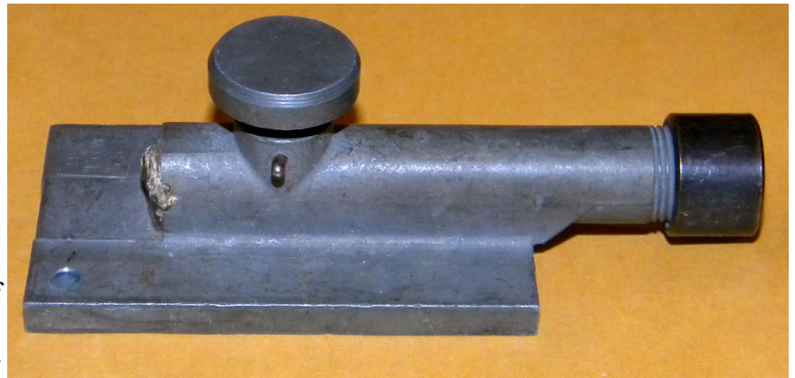
Switch, No. 2, Pressure, Mk. II, Side view
