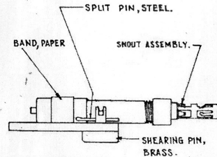
VIEW SHOWING SHEARING PIN. IN STOWED POSITION.
