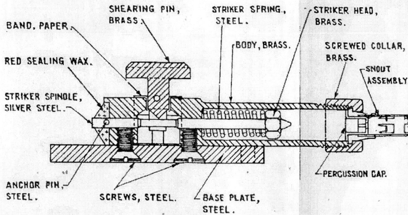
ENLARGED VIEW.
