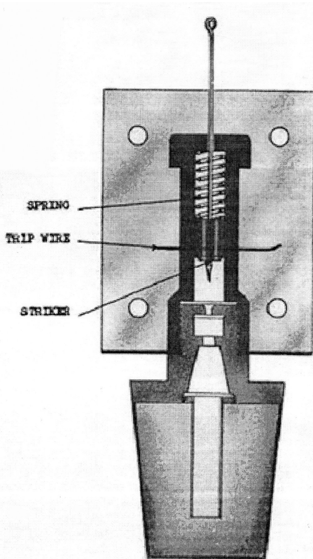
Diagram of Trip Mechanism No. 6 showing internal arrangement.
