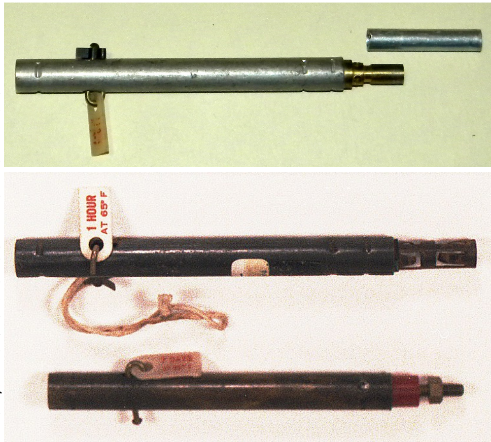
Top- Switch with early MD1 adapter and connecting sleeve
