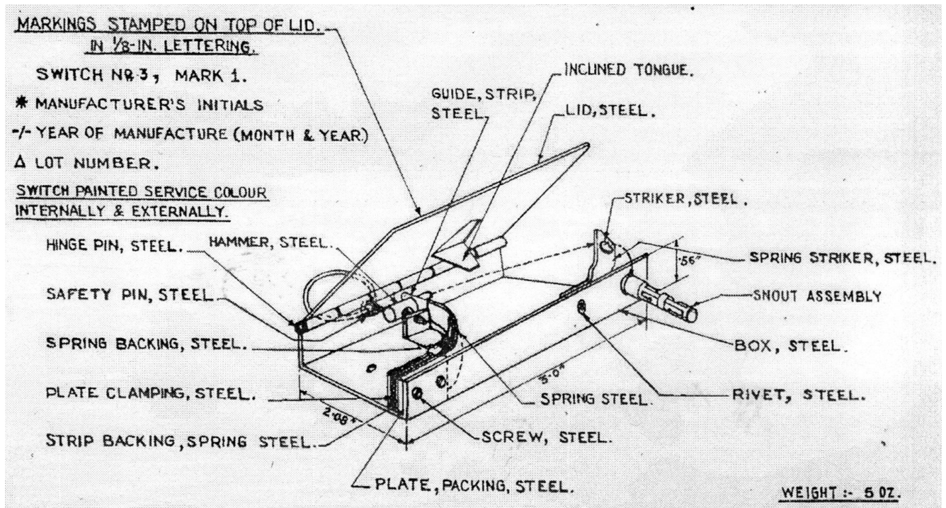
Internal Diagram of MD 1 Release Switch.
